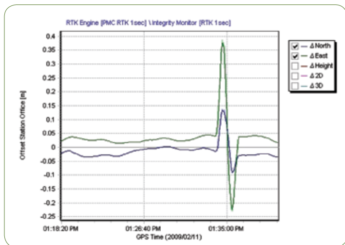
Fig. 11: To demonstrate the movement that can be detected, one of the stations was intentionally rocked from one side to the other.
